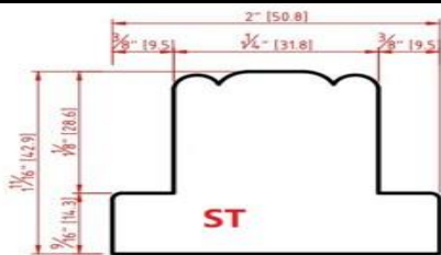
Small T-Post (ST)
