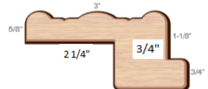
Large Z Frame (LZ)
