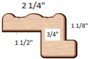
Jamestown Z Frame (JZ)
