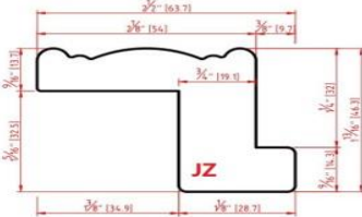
Jamestown Z Frame (JZ)
