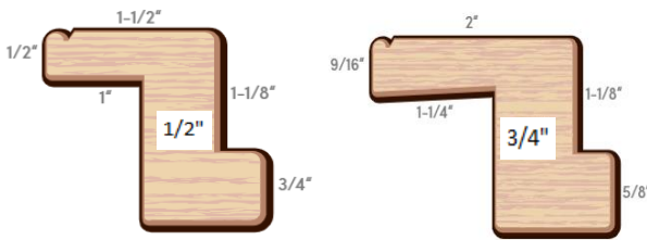
Small Z Frame (SZ) Beaded Z Frame (BZ)
