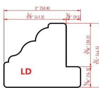
Large Deco (LD)
