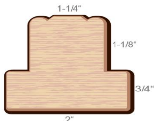
Small T-Post (ST)
