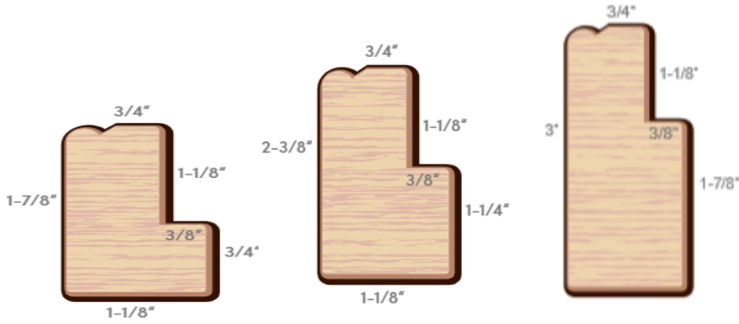
Small L Frame (SL) Medium L Frame (ML) Large L Frame (LL)
