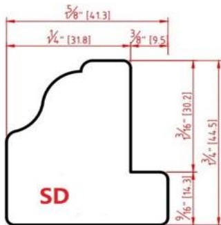
Small Deco (SD)
