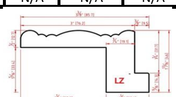
Large Z Frame (LZ)
