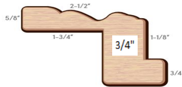
Colonial Z Frame (CZ)
