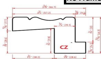
Colonial Z Frame (CZ)
