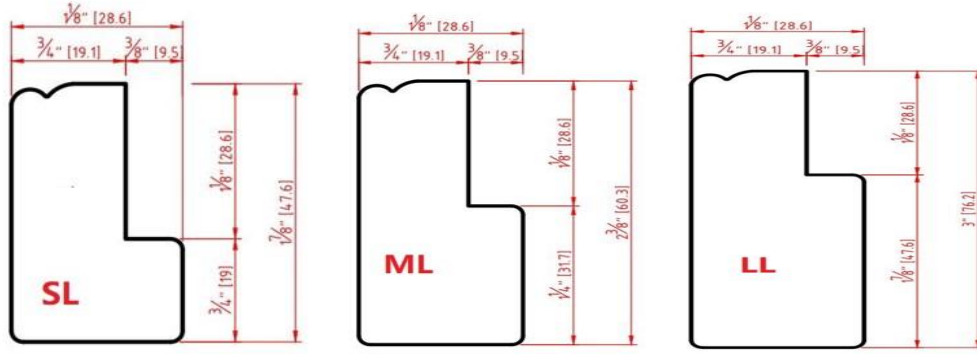
Small L Frame (SL)
