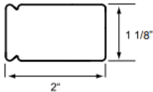
Square Stile
