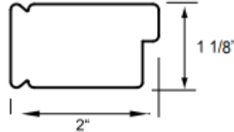
Rabbeted Stile
