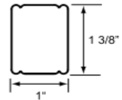
Standard Build-Out (BO) 1/4" Minimum
