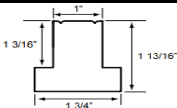
Small T-Post (STP)
