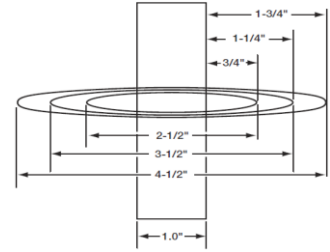
Depths needed for Louvers
