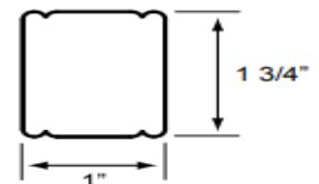
Standard Build-Out (BO) 1/4" Minimum
