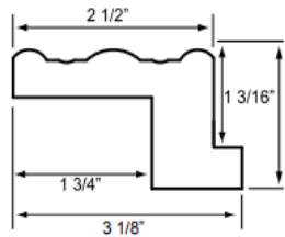
Medium Z-Frame (MDZ)
