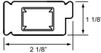
Rabbeted Stile
