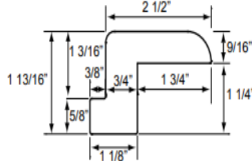
2" Flat Z-Frame (2FZ)
