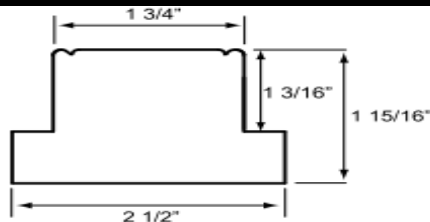
Large T-Post (LTP)
